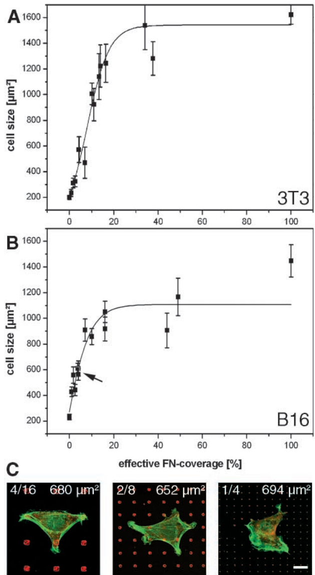
Fig. 9. Correlation between cell spreading and substratum coating. (A,B) The area covered by NIH/3T3 cells (A) and B16 cells (B) that have spread was plotted against the actual fibronectin surface for 12 different dot patterns, uncoated and homogeneously coated substrata. Bars represent s.e.m. (C) Three representative cells from patterns with 4% fibronectin coverage (arrow in B). Cell sizes as indicated in the upper right-hand corner were almost equal despite the different fibronectin patterns (actual length and margin to margin distance of dots is given in \mu\text{m} in the upper left corner).
